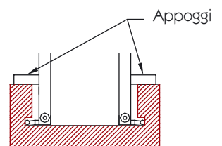
Controllo canalini e gole interne Inside channel and groove measurement
