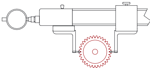
Controllo dentature esterne Outside tooth measurement
