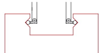
Controllo guide a "V" interne Inside "V" guide measurement
