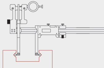
INSIDE CHANNEL AND GROOVE MEASUREMENT CONTROLLO CANALINI E GOLE INTERNE
