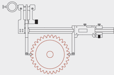
OUTSIDE TOOTH MEASUREMENT CONTROLLO DENTATURE ESTERNE
